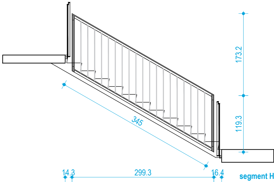
segment G
